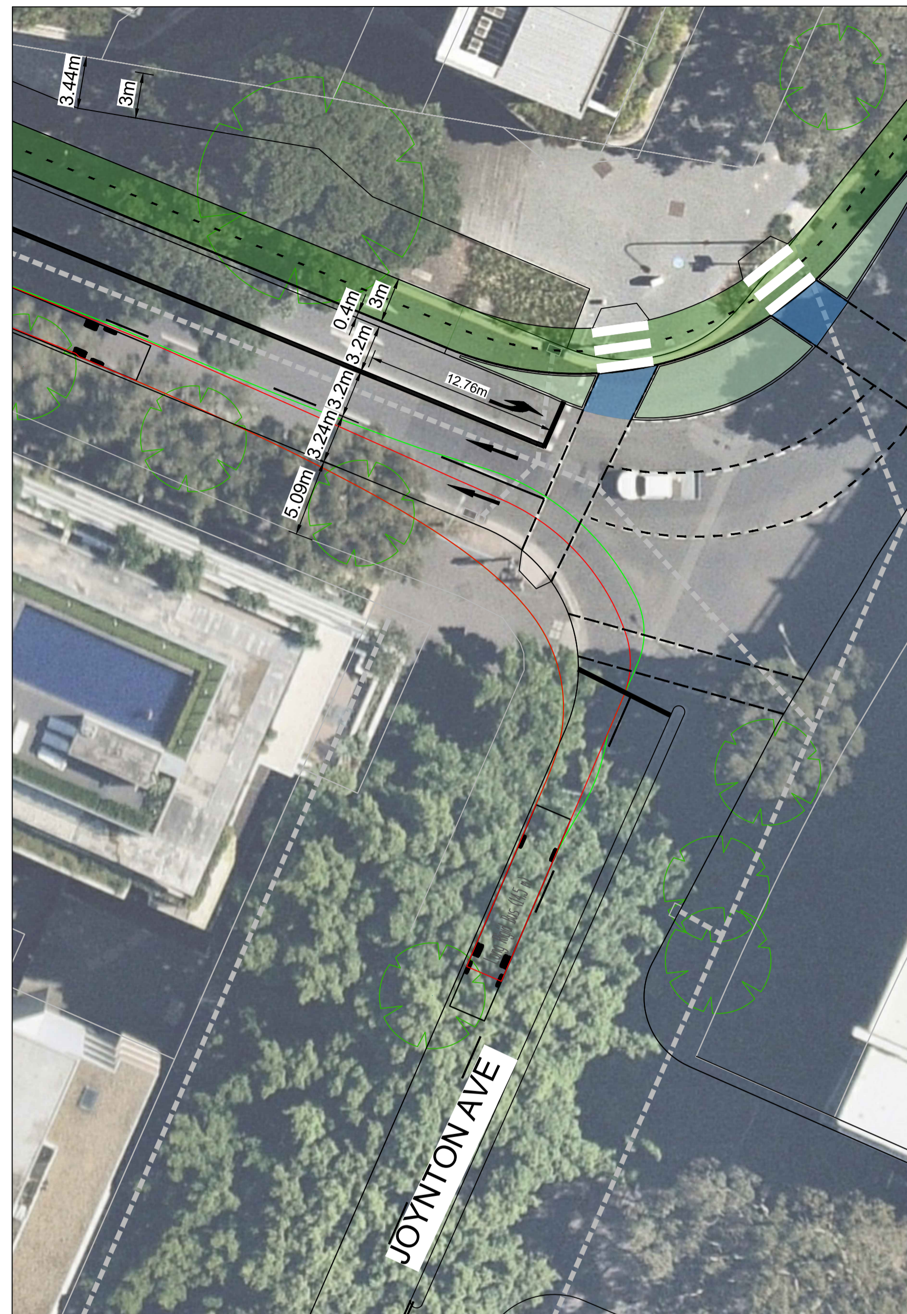
LONG RIGID BUS (14.5m) SCALE 1:250
