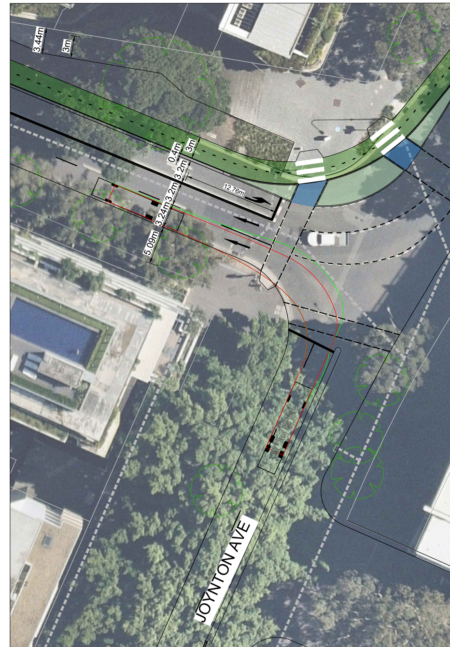
HEAVY RIGID VEHICLE (12.5m) SCALE 1:250
