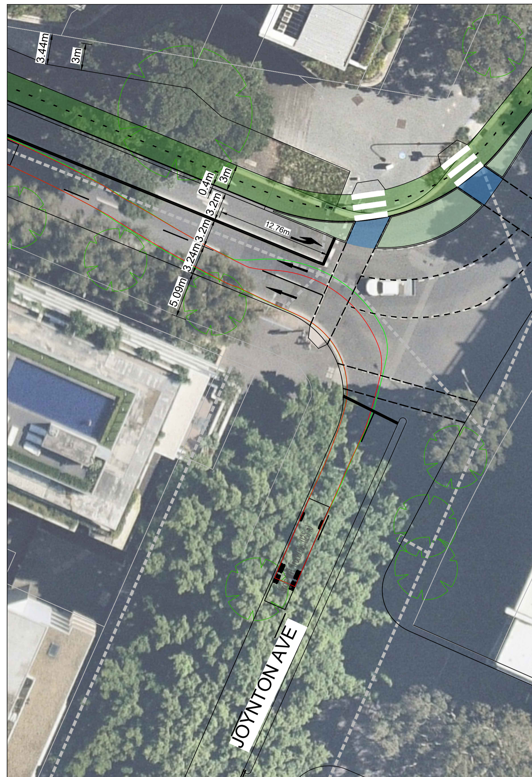
SINGLE UNIT TRUCK/BUS (12.5m) SCALE 1:250
